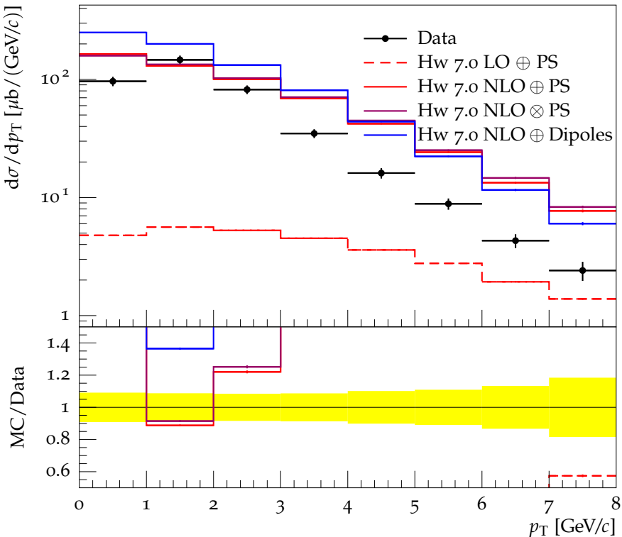
Prompt D^0 + \text{c.c.} d\sigma/dp_T for rapidity interval 2.5 < y < 3.0
