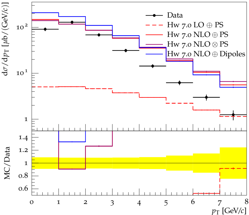
Prompt D^0 + \text{c.c.} d\sigma/dp_T for rapidity interval 3.0 < y < 3.5
