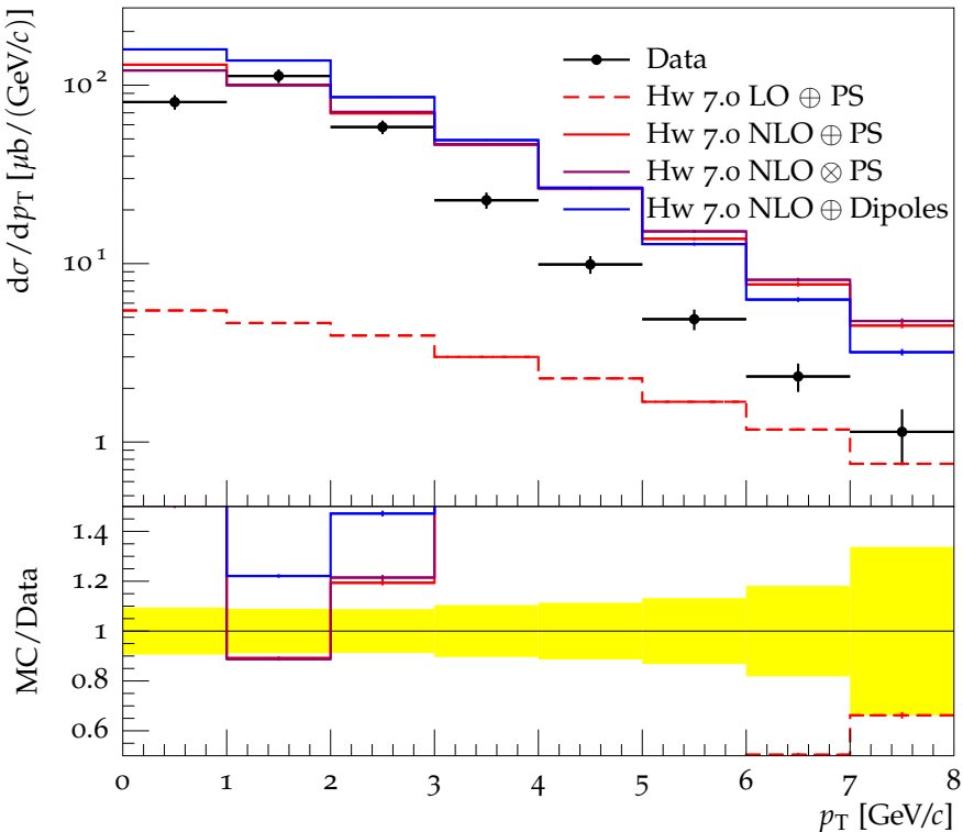
Prompt D^0 + \text{c.c.} d\sigma/dp_T for rapidity interval 3.5 < y < 4.0
