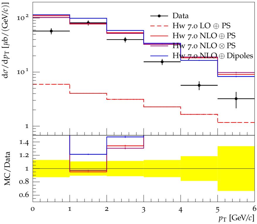
Prompt D^0 + \text{c.c.} d\sigma/dp_T for rapidity interval 4.0 < y < 4.5
