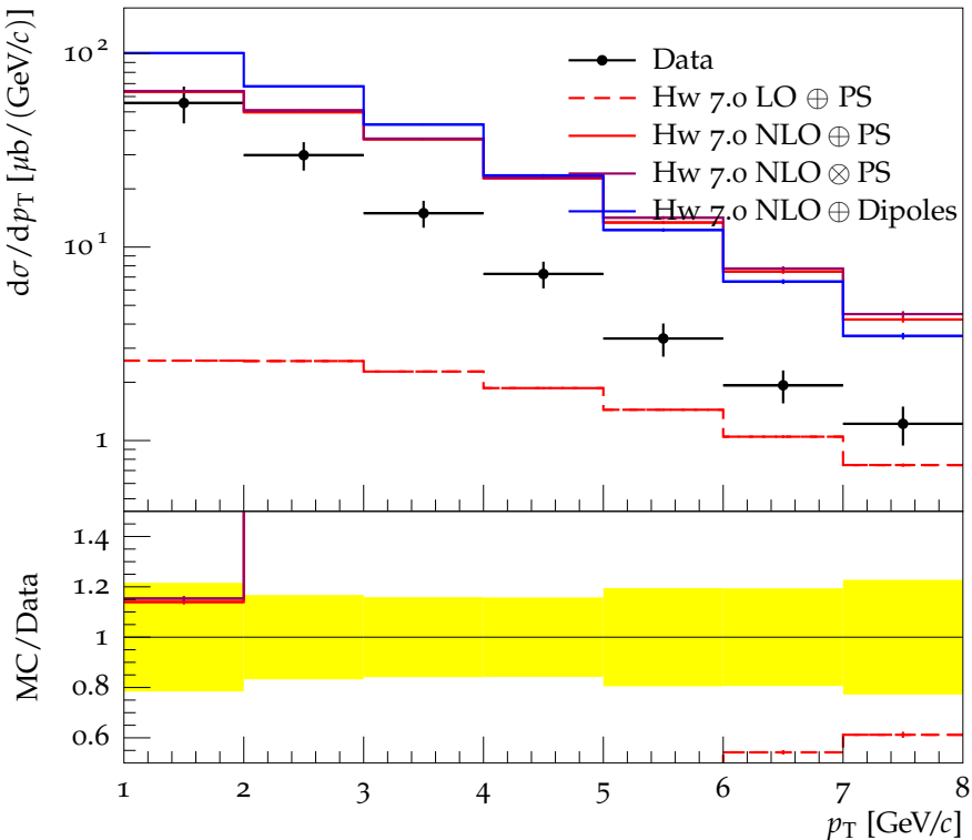
Prompt D^+ + \text{c.c.} d\sigma/dp_T for rapidity interval 2.0 < y < 2.5
