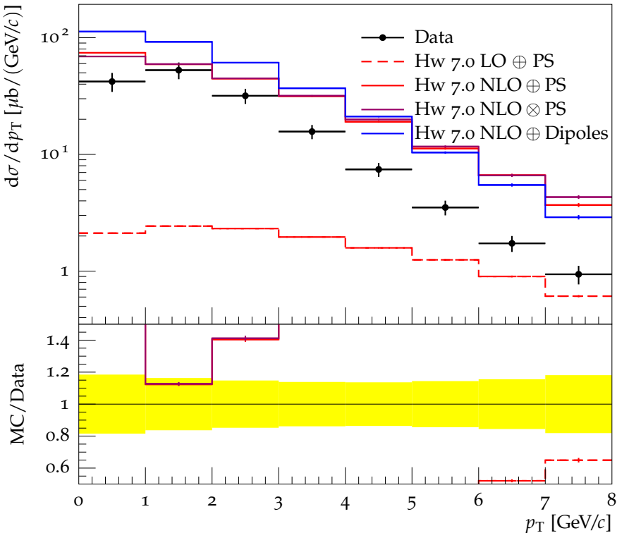
Prompt D^+ + \text{c.c.} d\sigma/dp_T for rapidity interval 2.5 < y < 3.0
