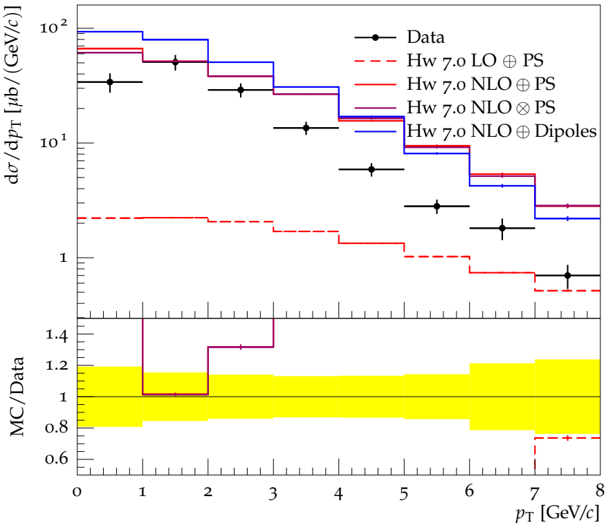
Prompt D^+ + \text{c.c.} d\sigma/dp_T for rapidity interval 3.0 < y < 3.5
