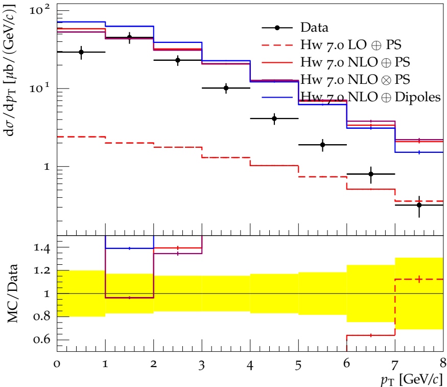
Prompt D^+ + \text{c.c.} d\sigma/dp_T for rapidity interval 3.5 < y < 4.0
