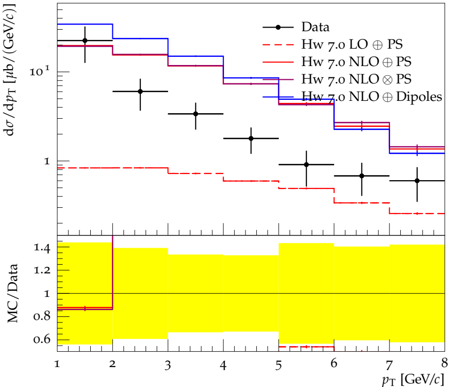
Prompt D_s^+ + \text{c.c.} d\sigma/dp_T for rapidity interval 2.0 < y < 2.5
