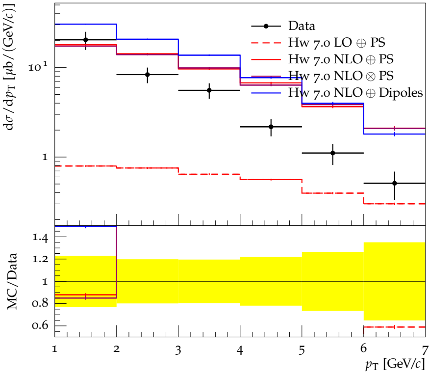
Prompt D_s^+ + \text{c.c.} d\sigma/dp_T for rapidity interval 2.5 < y < 3.0
