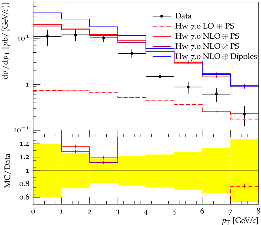
Prompt D_s^+ + \text{c.c.} d\sigma/dp_T for rapidity interval 3.0 < y < 3.5
