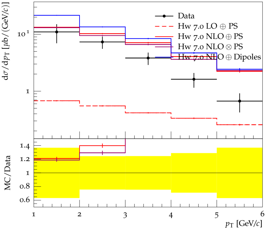
Prompt D_s^+ + c.c. d\sigma/dp_T for rapidity interval 3.5 < y < 4.0
