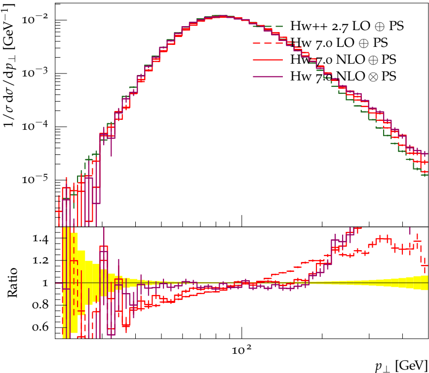
Transverse momentum distribution for jet 1
