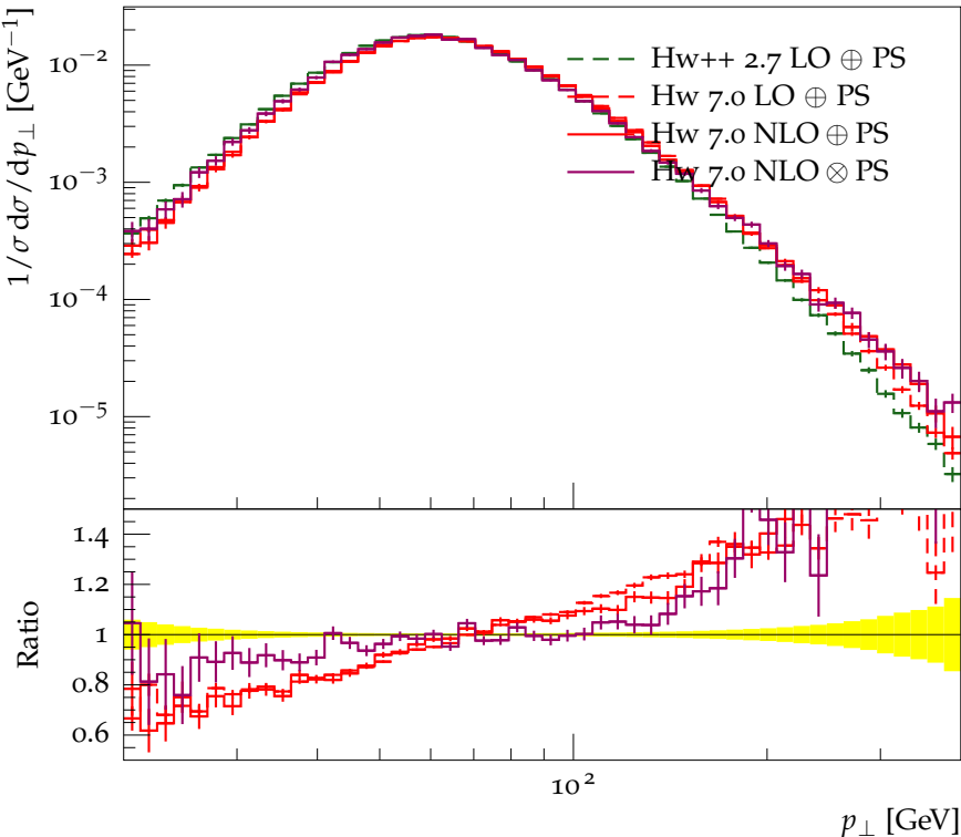
Transverse momentum distribution for jet 2
