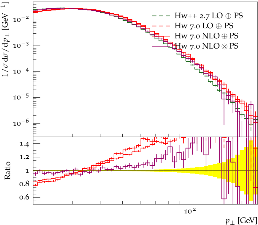
Transverse momentum distribution for jet 4
