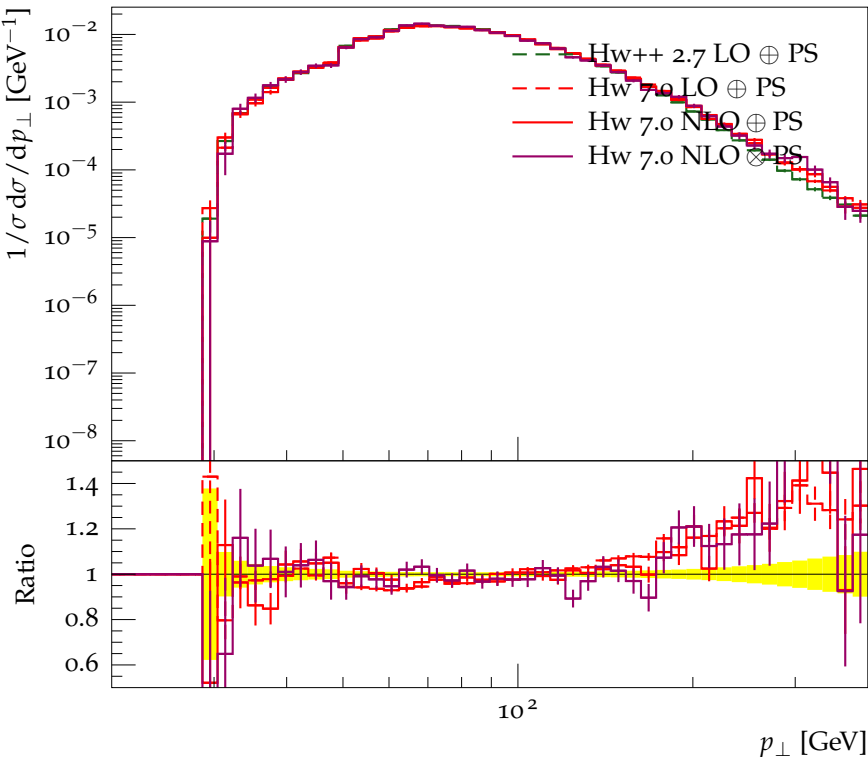
Transverse momentum distribution for b -jet 1
