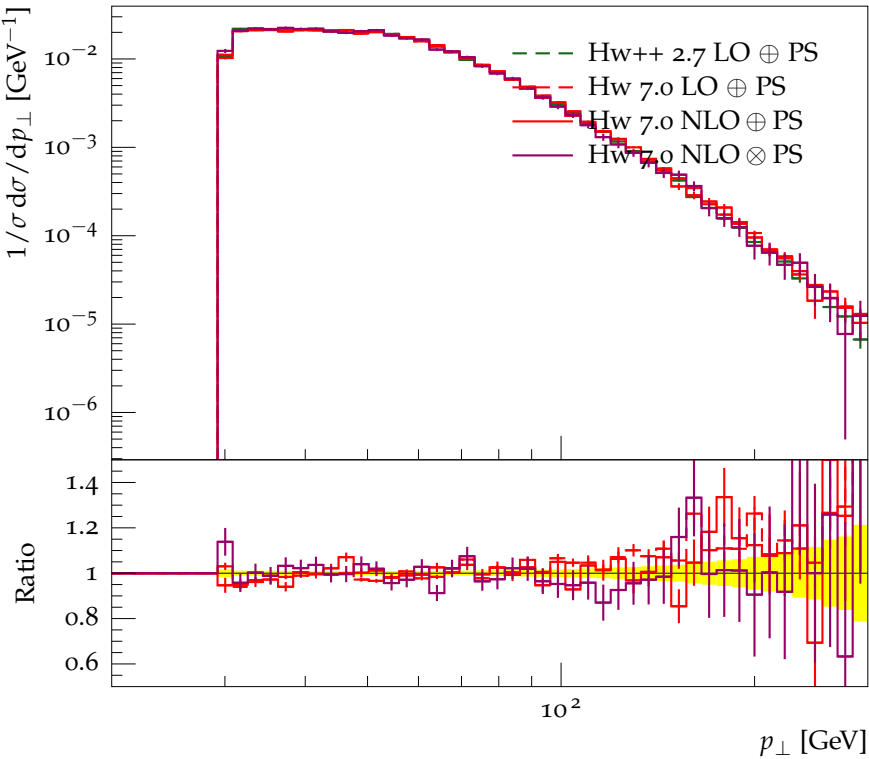
Transverse momentum distribution for b -jet 2
