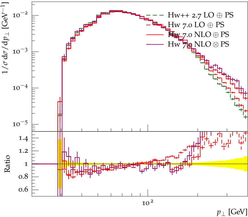
Transverse momentum distribution for light jet 1
