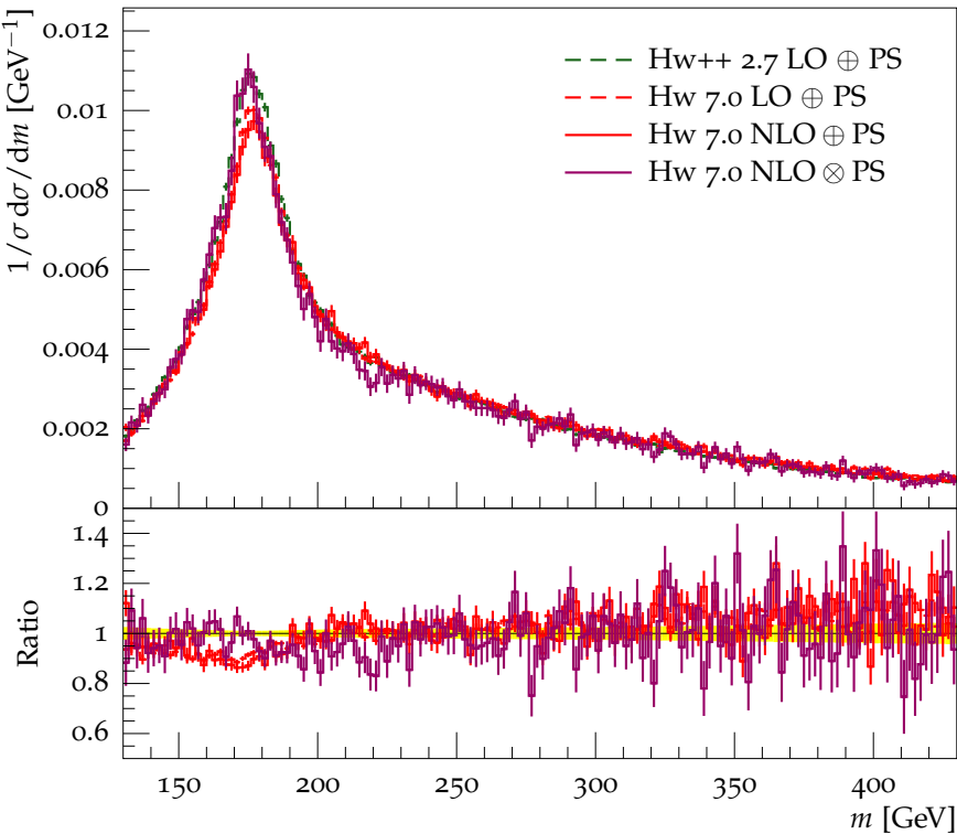
Mass distribution for reconstructed top
