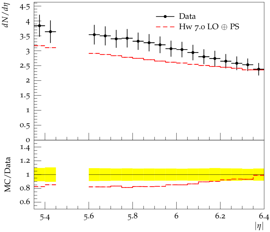
Charged particle |\eta| at 7 TeV, track p_{\perp} > 40 MeV, for N_{\text{ch}} \geq 1
