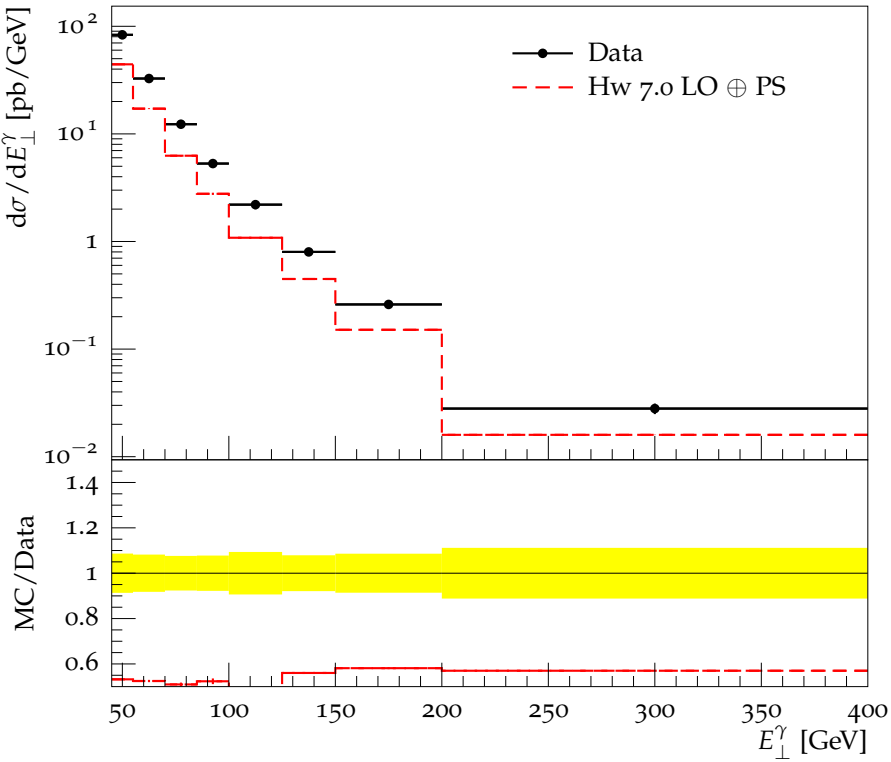
Transverse energy of isolated prompt photon, |\eta| < 0.6
