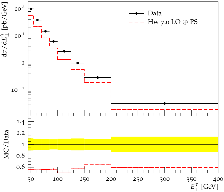
Transverse energy of isolated prompt photon, 0.6 < |\eta| < 1.37
