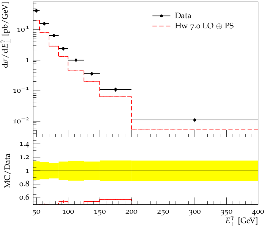
Transverse energy of isolated prompt photon, 1.52 \leq |\eta| < 1.81
