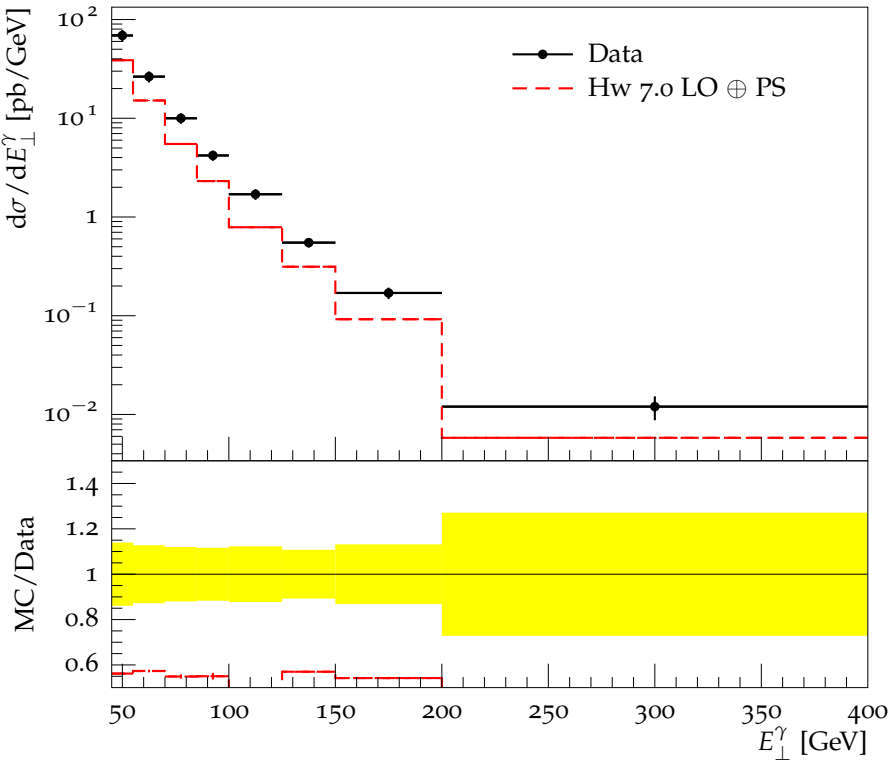
Transverse energy of isolated prompt photon, 1.81 \leq |\eta| < 2.37
