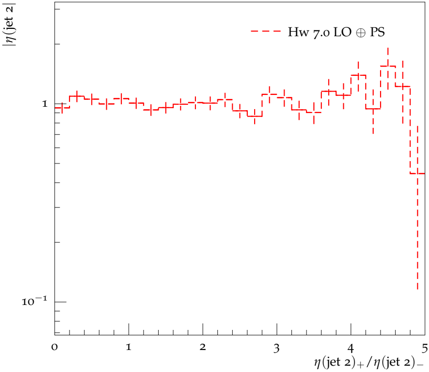
Pseudorapidity +/- ratio of second jet
