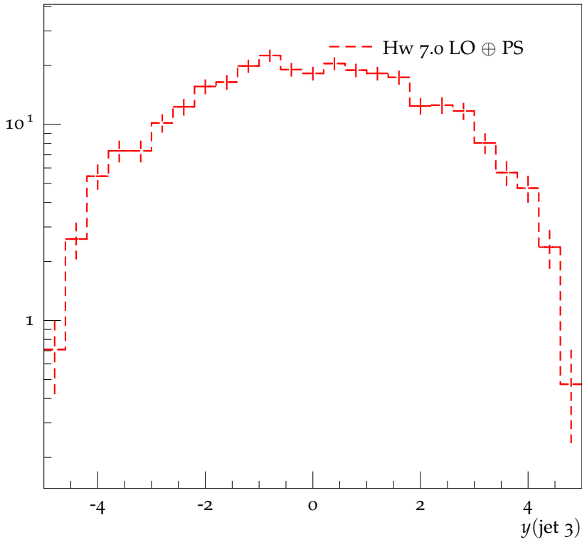
Rapidity of third jet
