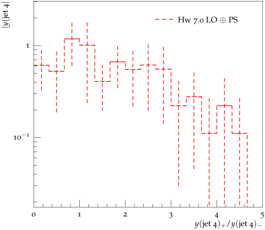
Rapidity +/- ratio of fourth jet
