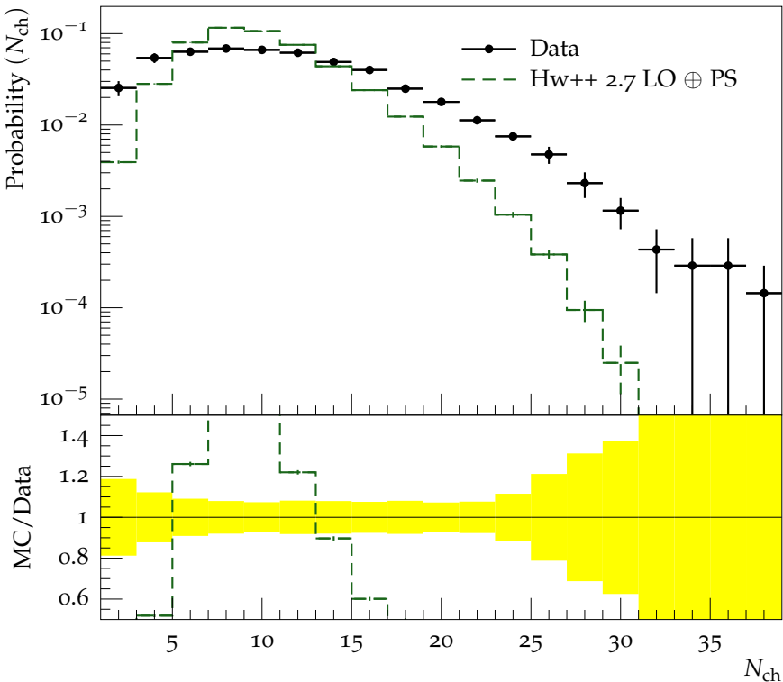
Charged multiplicity at \sqrt{s} = 44.5 GeV (inelastic events)
