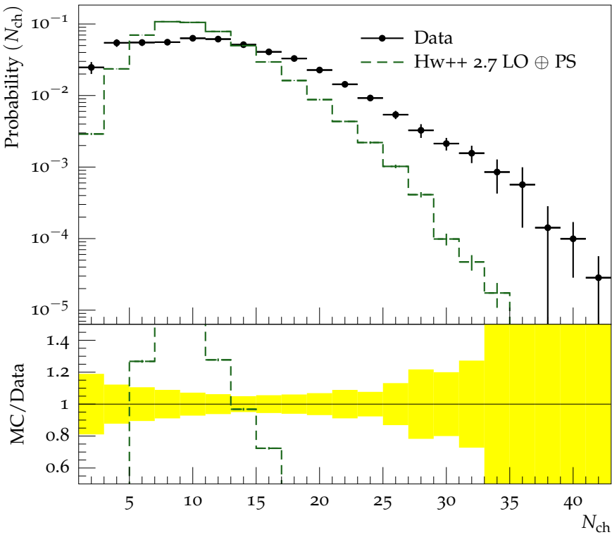
Charged multiplicity at \sqrt{s} = 52.6 GeV (inelastic events)
