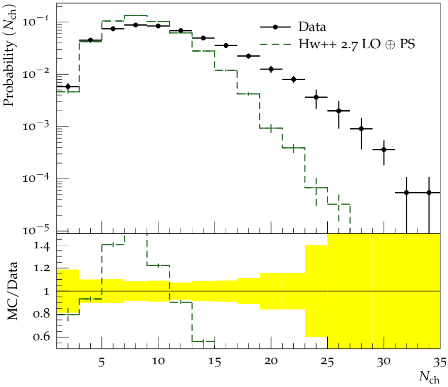
Charged multiplicity at \sqrt{s} = 30.4 GeV (NSD events)
