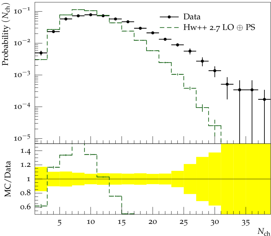
Charged multiplicity at \sqrt{s} = 44.5 GeV (NSD events)
