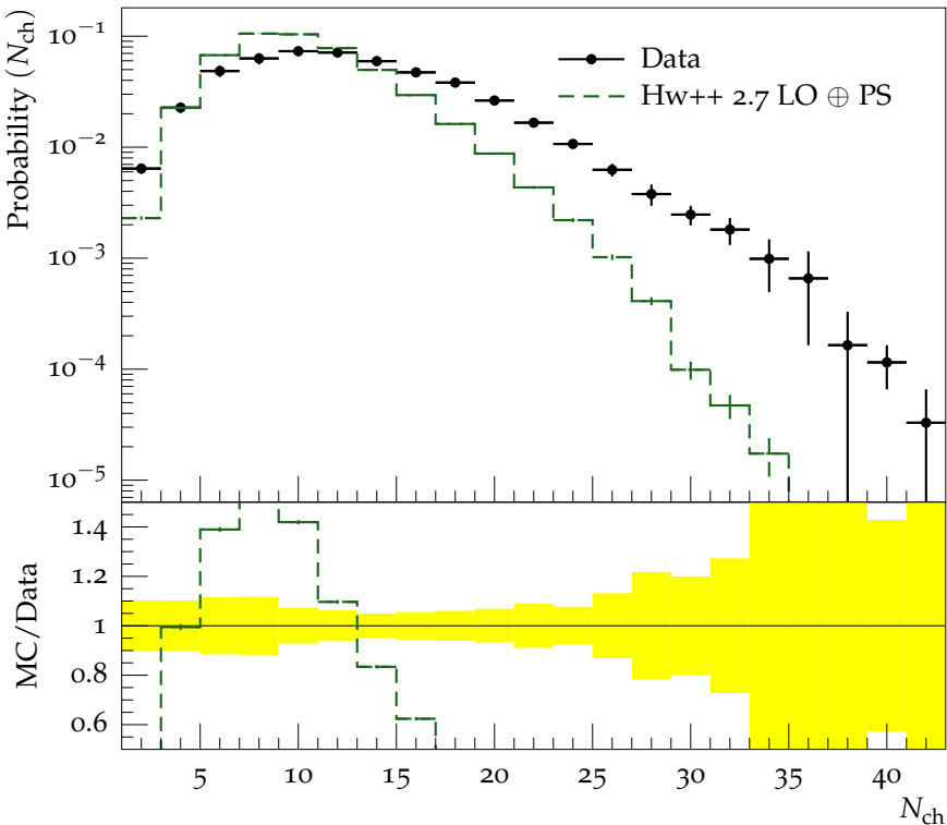
Charged multiplicity at \sqrt{s} = 52.6 GeV (NSD events)
