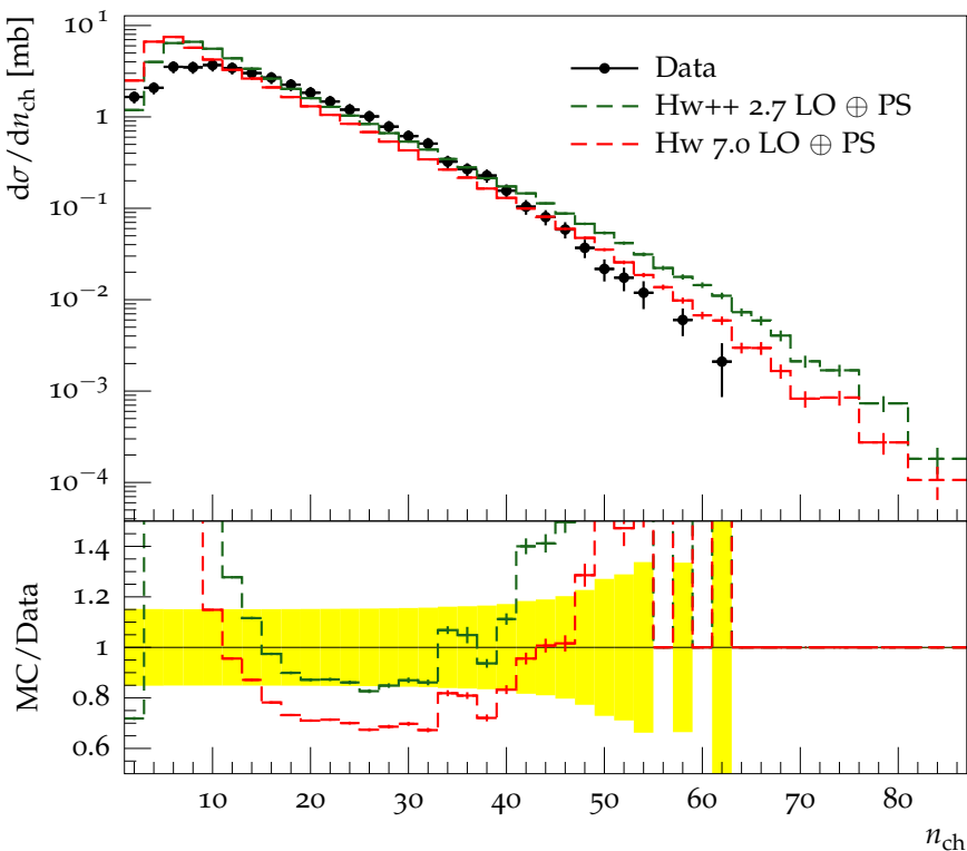
Multiplicity distribution at \sqrt{s} = 200\text{GeV}
