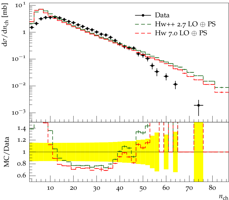
Multiplicity distribution at \sqrt{s} = 500\text{GeV}
