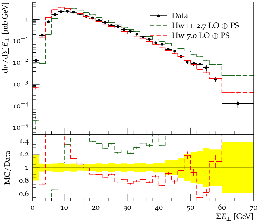
Transverse energy cross section at \sqrt{s} = 200\text{GeV} and |\eta| < 6
