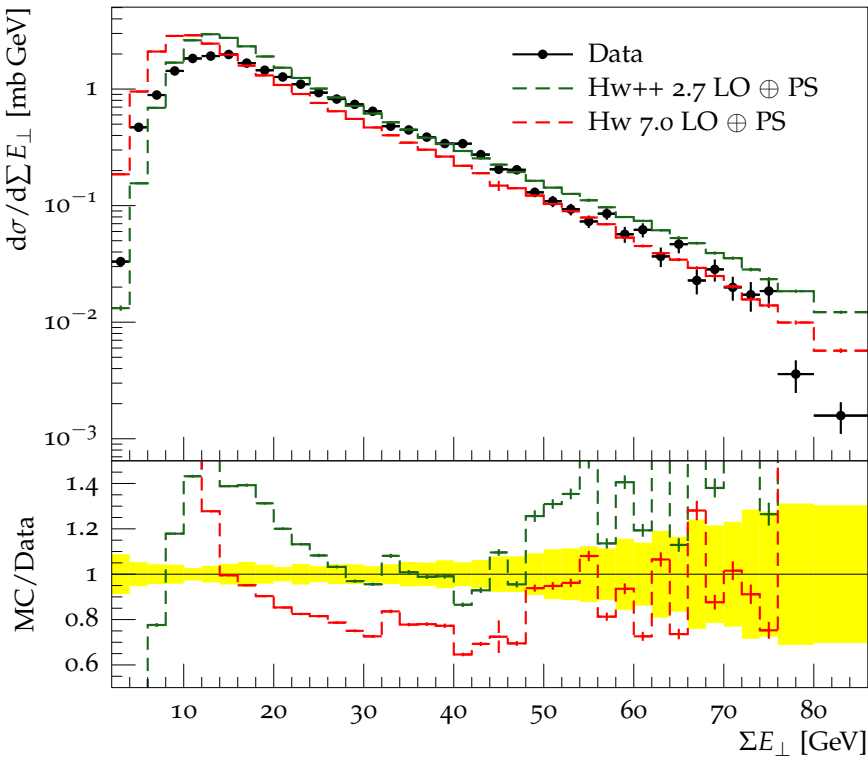
Transverse energy cross section at \sqrt{s} = 500\text{GeV} and |\eta| < 6
