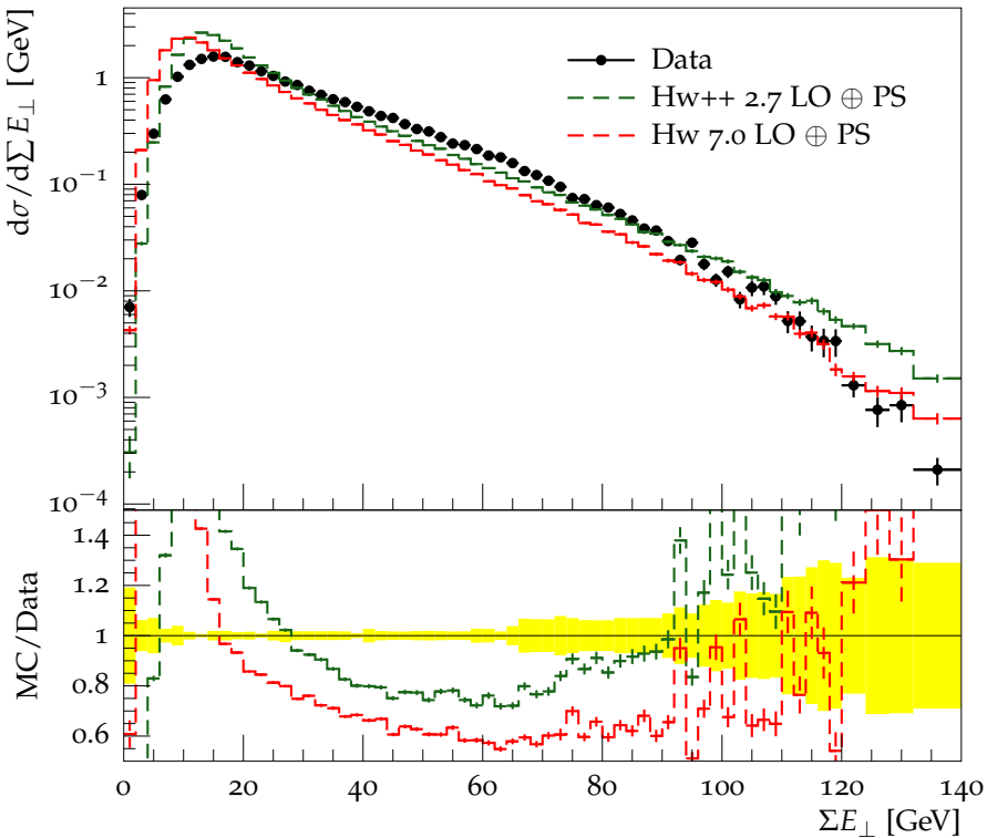
Transverse energy cross section at \sqrt{s} = 900\text{GeV} and |\eta| < 6
