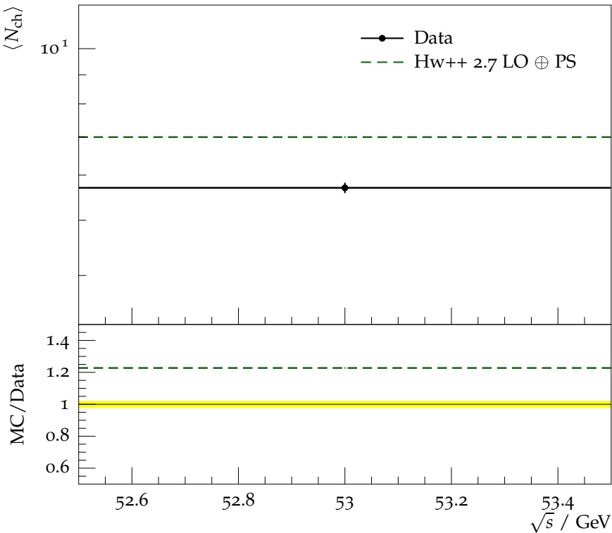
Mean charged multiplicity for p\bar{p} collisions at \sqrt{s} = 53 GeV
