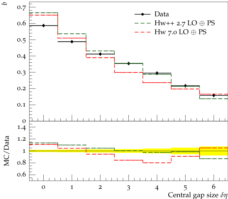
Forward-backward correlation b vs. gap size \sqrt{s} = 546 GeV
