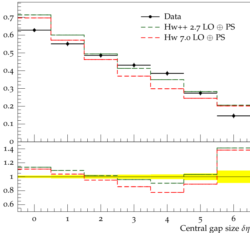
Forward-backward correlation b vs. gap size \sqrt{s} = 900 GeV
