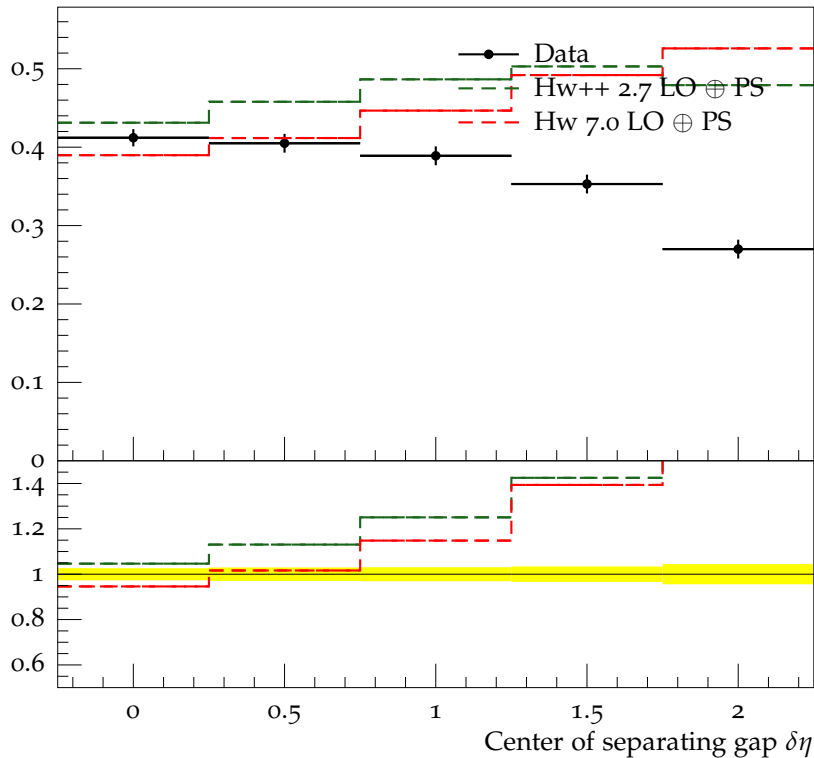
Forward-backward correlation b vs. gap center \sqrt{s} = 546 GeV
