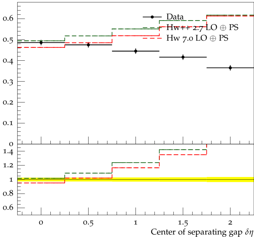
Forward-backward correlation b vs. gap center \sqrt{s} = 900 GeV
