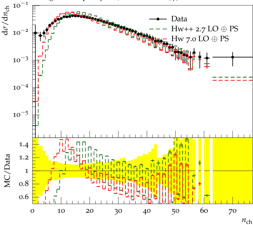
Charged multiplicity at \sqrt{s} = 200 GeV, |\eta| < 5.0
