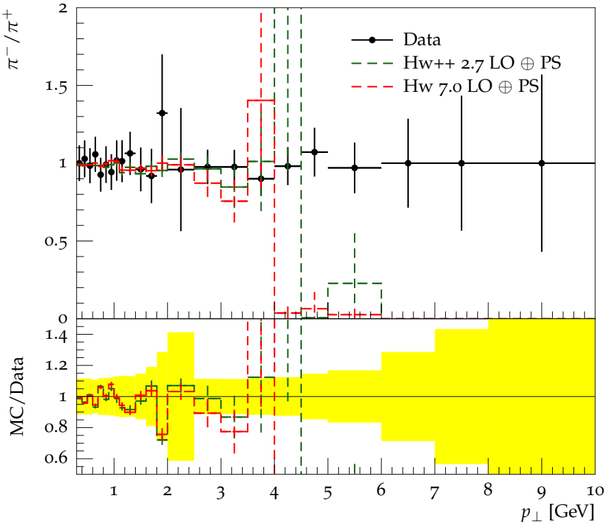
Ratio of \pi^-/\pi^+ as function of p_\perp
