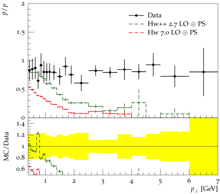
Ratio of \bar{p}/p as function of p_{\perp}
