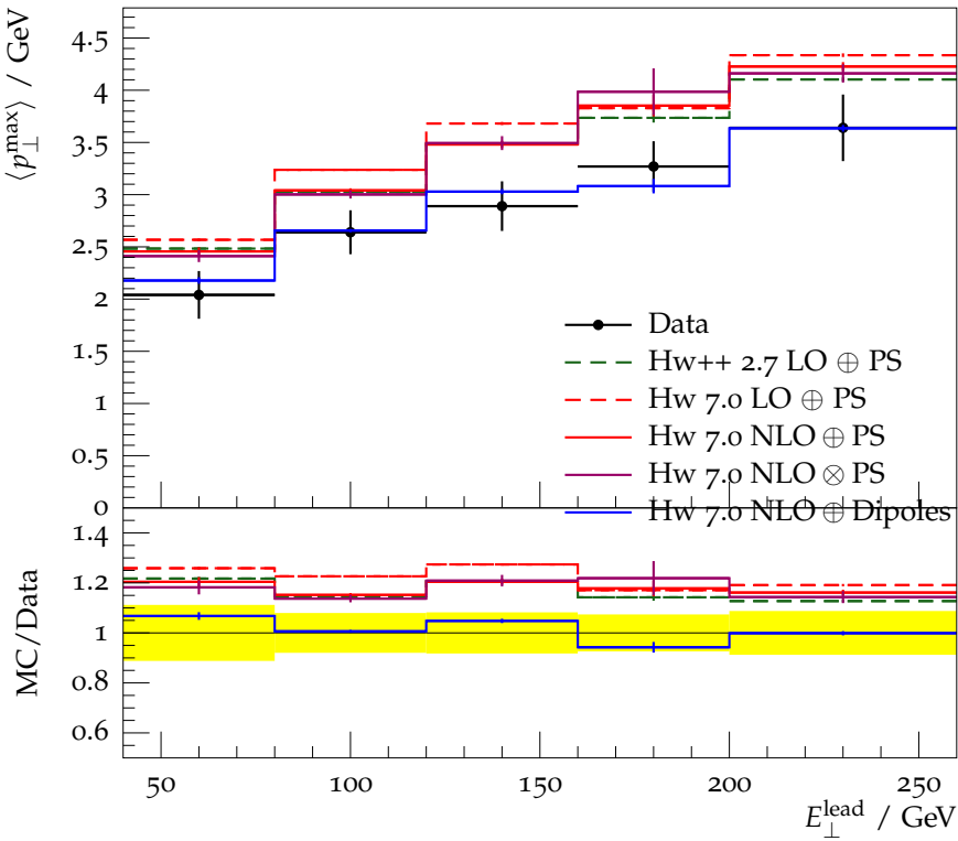
Transverse cone \langle\langle p_{\perp}^{\max} \rangle\rangle vs. E_{\perp}^{\text{lead}} at \sqrt{s} = 1800 GeV
