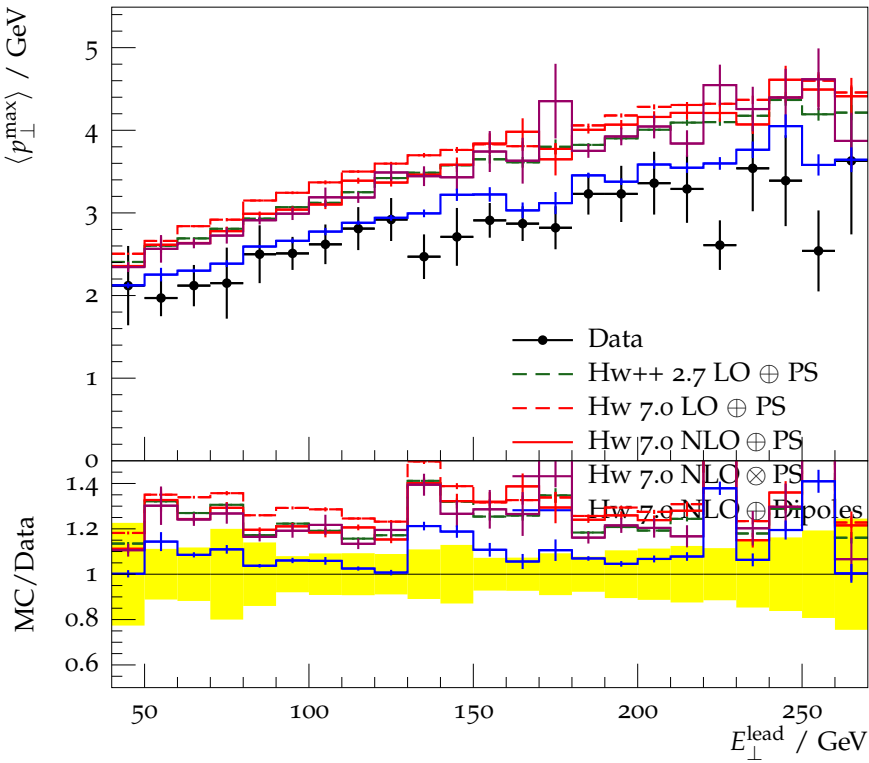
Transverse cone \langle p_{\perp}^{\max} \rangle vs. E_{\perp}^{\text{lead}} at \sqrt{s} = 1800 GeV
