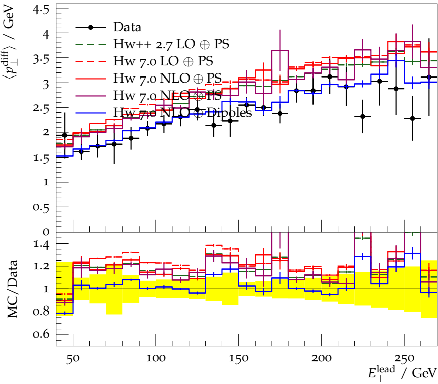
Transverse cone \langle p_{\perp}^{\text{diff}} \rangle vs. E_{\perp}^{\text{lead}} at \sqrt{s} = 1800 GeV
