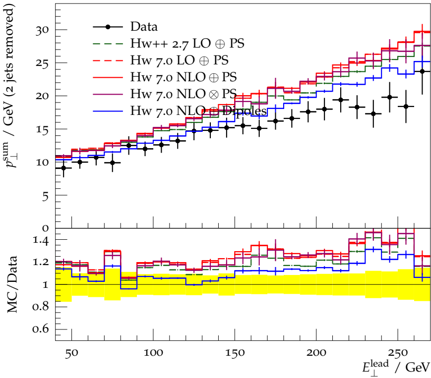
Swiss Cheese p_{\perp}^{\text{sum}} vs. E_{\perp}^{\text{lead}} (2 jets removed) at \sqrt{s} = 1800 GeV
