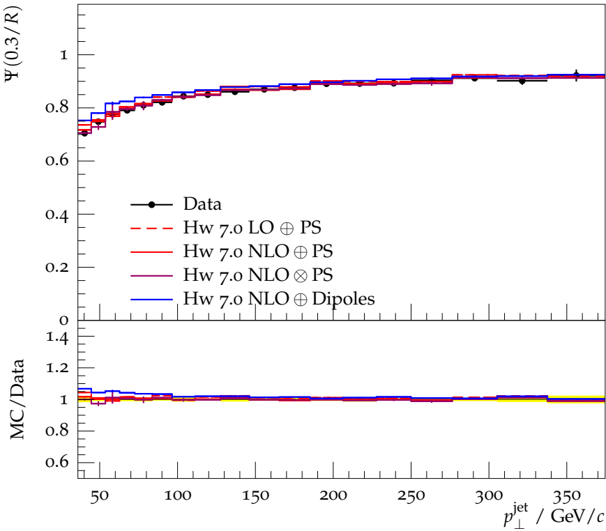
Integral jet shape, \Psi(0.3/R) , vs. p_{\perp}^{\text{jet}}
